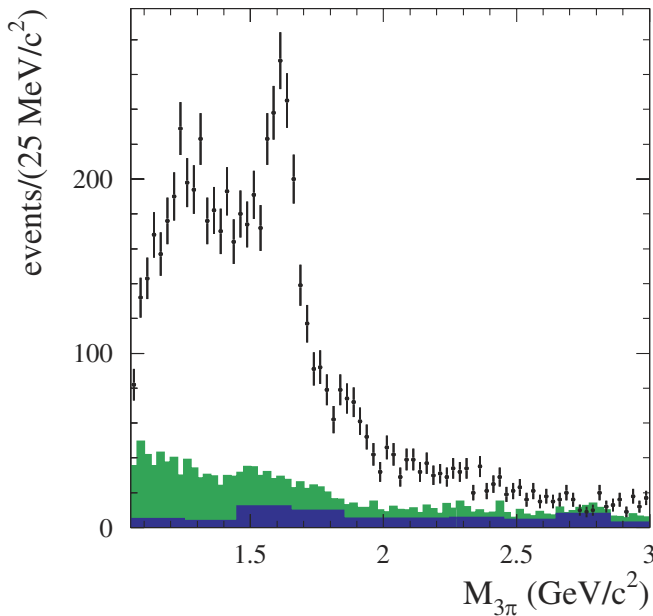
FIG. 5 (color online). The 3\pi mass spectrum for data events with \chi^2 < 40 . The lightly shaded histogram shows the mass spectrum for calculated background. The dark histogram is e^+e^- \rightarrow \pi^+\pi^-\pi^0\pi^0 background.
