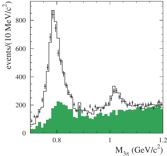
FIG. 11 (color online). The 3\pi mass spectrum for events with 40 < \chi^2 < 500 . Points with error bars show the data distribution. The solid line shows the sum of the distributions for simulated e^+e^- \rightarrow \pi^+\pi^-\pi^0\gamma and background processes. The shaded histogram shows the distribution for background processes.
