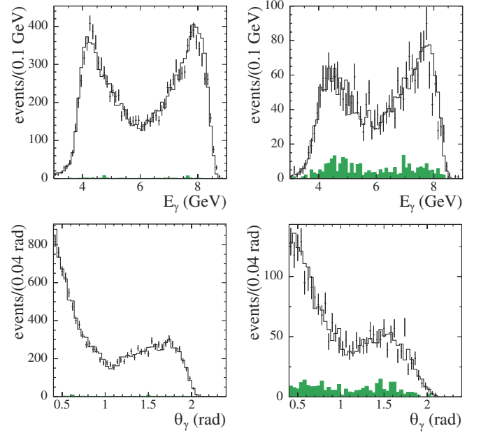
FIG. 13 (color online). Distributions of the ISR photon energy (1st row) and polar angle (2nd row) for data (points with error bars) and simulation (solid line) events with \chi^2 < 20 . The left and right columns correspond to the mass regions 0.75 < M_{3\pi} < 0.82 \text{GeV}/c^2 and 1.40 < M_{3\pi} < 1.80 \text{GeV}/c^2 , respectively. Shaded histograms show the calculated background contributions.
