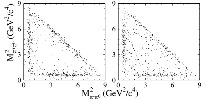
FIG. 20. The Dalitz plot for J/\psi \rightarrow 3\pi candidates in data (left) and simulation (right).
