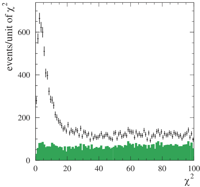
FIG. 3 (color online). The \chi^2 distributions for data from the mass range 1.05 < M_{3\pi} < 3.00 GeV/c 2 . The shaded histogram shows events rejected by background suppression cuts.
