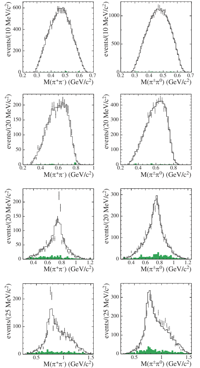
FIG. 15 (color online). Distributions of \pi^+\pi^- (left column) and \pi^+\pi^0 (right column) invariant masses for data (points with error bars) and simulation (solid line) for events with \chi^2 < 20 . The rows correspond to the mass regions: 0.75 < M_{3\pi} < 0.82 \text{ GeV}/c^2 (1st row), 1.00 < M_{3\pi} < 1.04 \text{ GeV}/c^2 (2nd row), 1.10 < M_{3\pi} < 1.40 \text{ GeV}/c^2 (3rd row), and 1.40 < M_{3\pi} < 1.80 \text{ GeV}/c^2 (4th row). Shaded histograms show the calculated background contributions.
