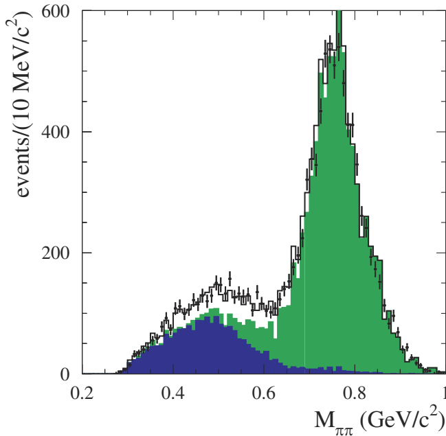
FIG. 7 (color online). \pi^+\pi^- invariant mass spectrum for events with 100 < \chi^2 < 500 and 0.85 < M_{3\pi} < 1.05 GeV/c 2 . The points with error bars are data. The histogram is the sum of spectra for simulated events of e^+e^- \rightarrow \pi^+\pi^-\pi^0\gamma and background processes. The lightly shaded histogram is the sum of all background processes. The difference between the dark and lightly shaded histogram shows the e^+e^- \rightarrow \pi^+\pi^-\gamma contribution.
