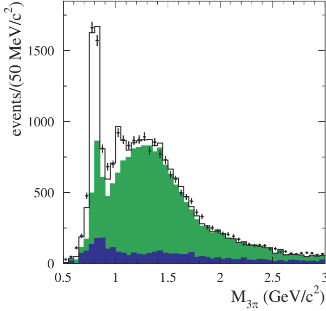
FIG. 6 (color online). The M_{3\pi} spectrum for events with 100 < \chi^2 < 500 and E_{\pi^0} > 1 GeV. The points with error bars are data. The histogram is the sum of spectra for simulated events of e^+e^- \rightarrow \pi^+\pi^-\pi^0\gamma and background processes. The lightly shaded histogram is the sum of all background processes. The difference between the dark and lightly shaded histograms shows the e^+e^- \rightarrow \pi^+\pi^-\pi^0\pi^0\gamma contribution.
