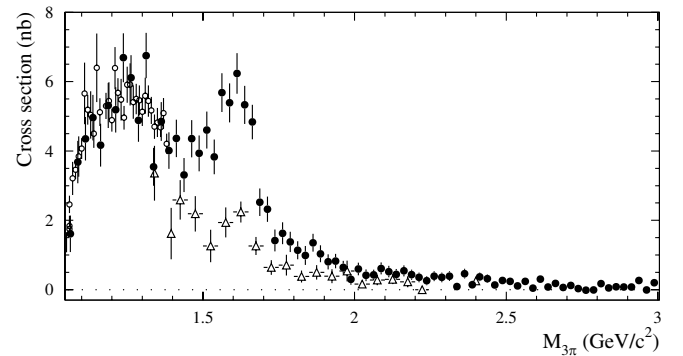
FIG. 18. The e^+e^- \rightarrow \pi^+\pi^-\pi^0 cross section measured in this work (filled circles), by SND (open circles), and DM2 (open triangles).
