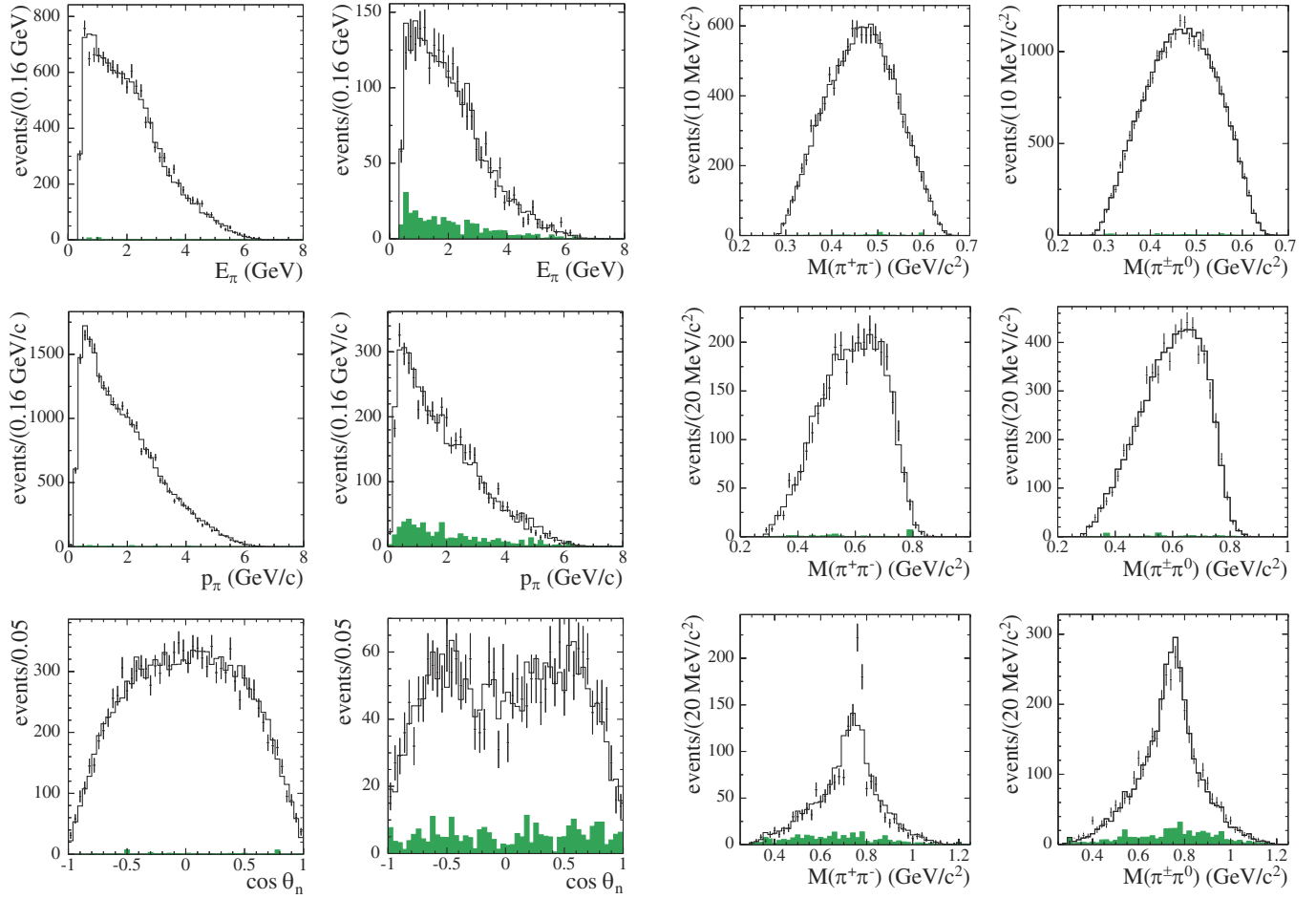
FIG. 14 (color online). Distributions of \pi^0 energy (1st row), charged-pion momentum (2nd row), and angle between the normal to the 3\pi plane in the three-pion rest frame and the direction of the 3\pi system in the laboratory frame (3rd row) for data (points with error bars) and simulation (solid line) events with \chi^2 < 20 . The left and right columns correspond to the mass regions 0.75 < M_{3\pi} < 0.82 \text{ GeV}/c^2 and 1.40 < M_{3\pi} < 1.80 \text{ GeV}/c^2 , respectively. Shaded histograms show the calculated background contributions.
