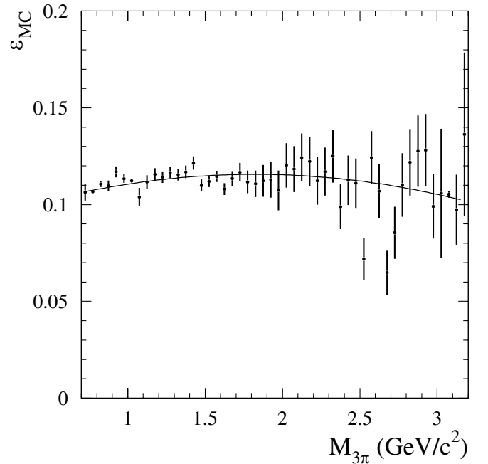
FIG. 10. The 3\pi mass dependence of the detection efficiency obtained from MC simulation. The line is the fit to a second-order polynomial.
