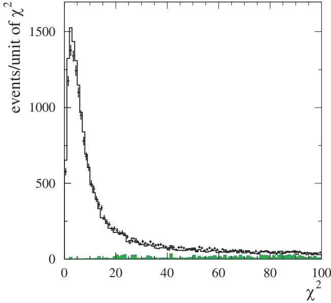
FIG. 2 (color online). The \chi^2 distributions for data (points with error bars) and simulated (histogram) events from the \omega mass region. The shaded histogram shows the distribution for simulated background events.
